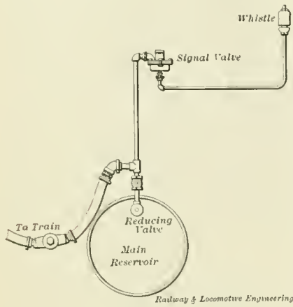
FIG. 1.—SIGNAL PIPING.
